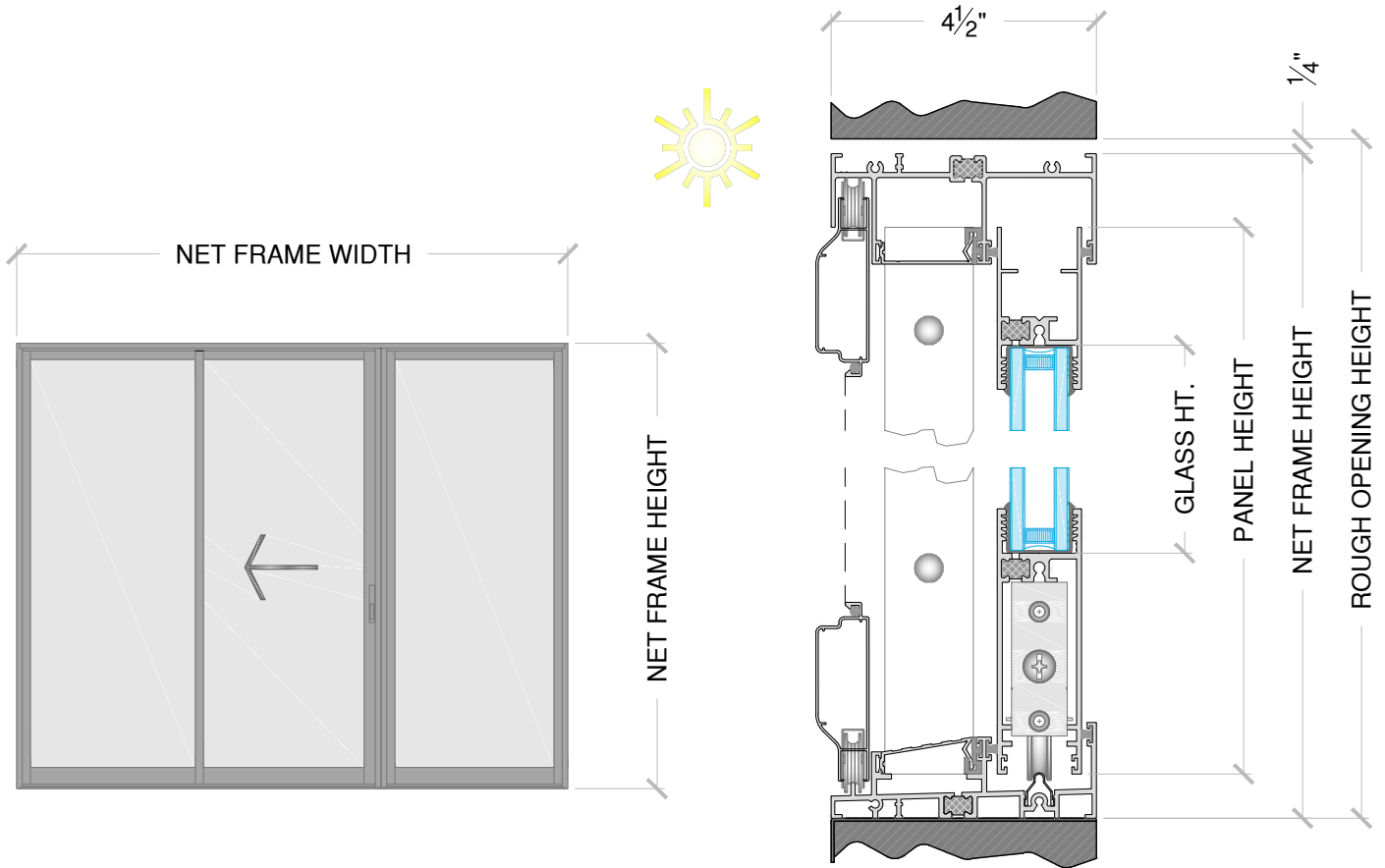
Section
