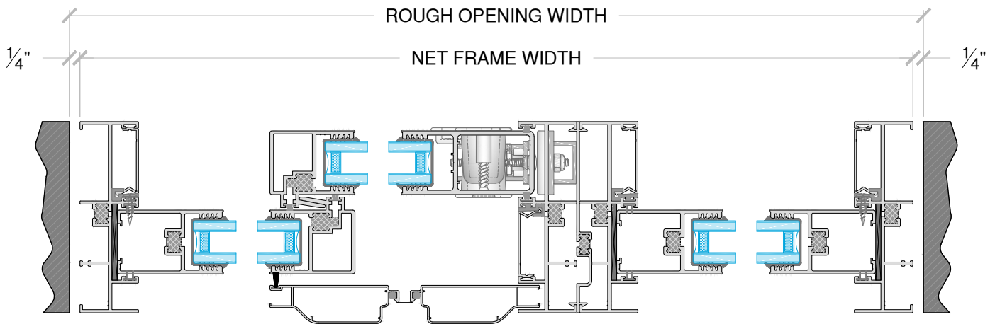
Section
