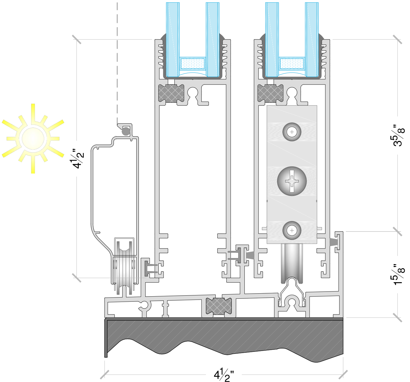
5a Standard Slide Sill w/ 4.50" Rail
