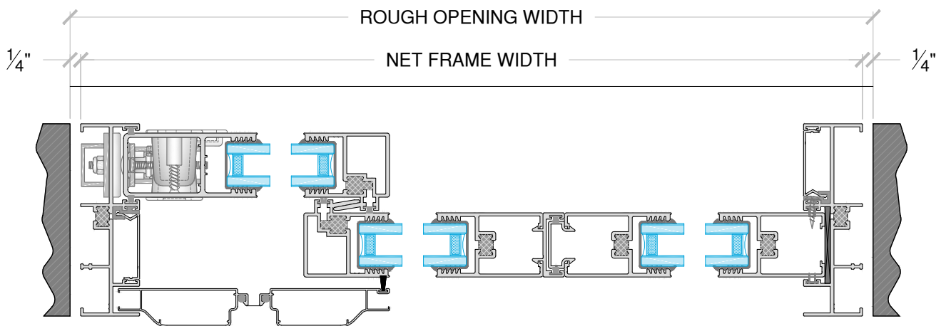
Section
