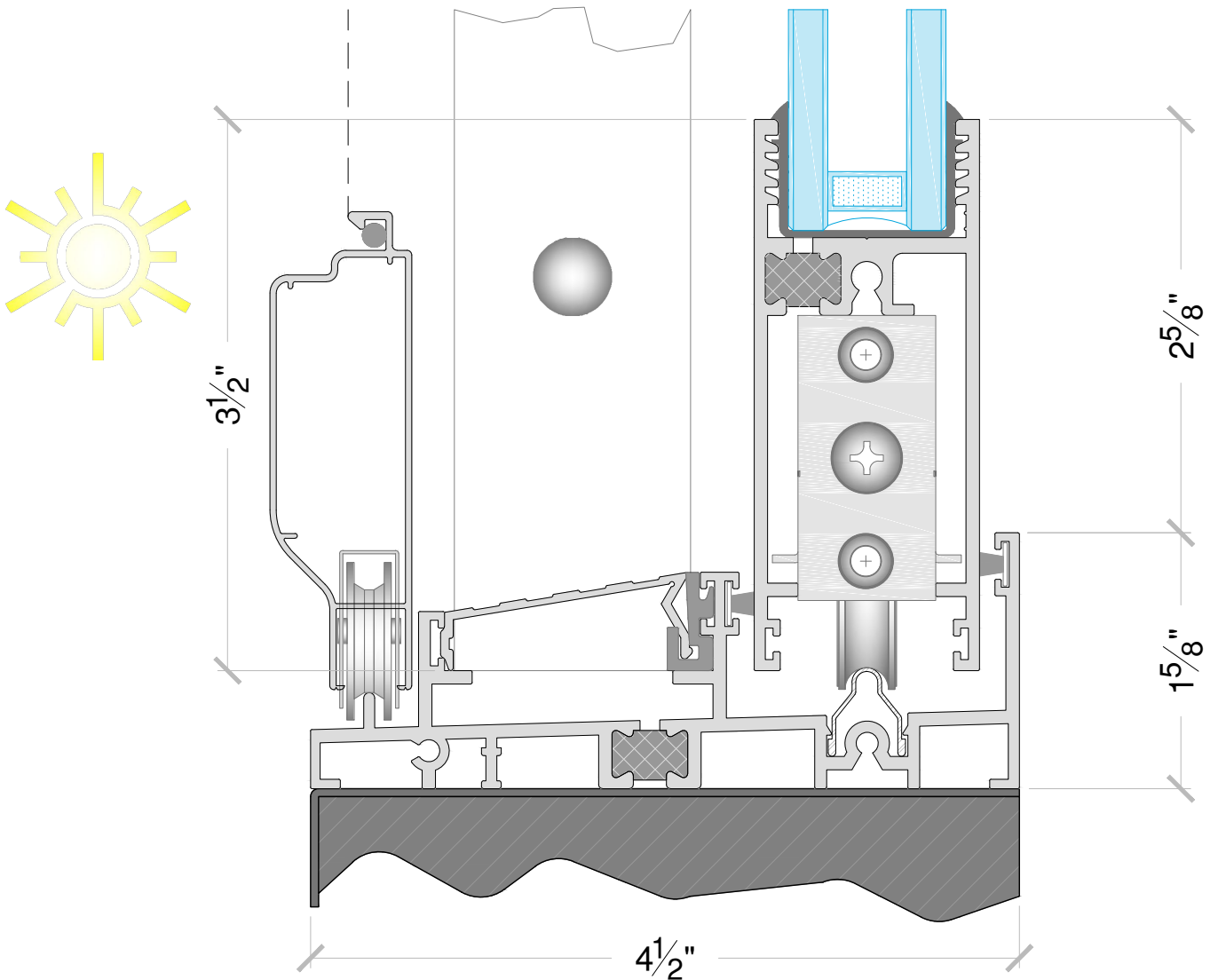
5b Standard Slide Sill w/ 3.50" Rail
