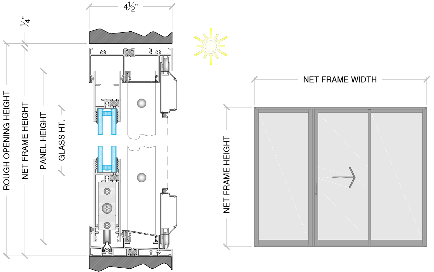
Section
