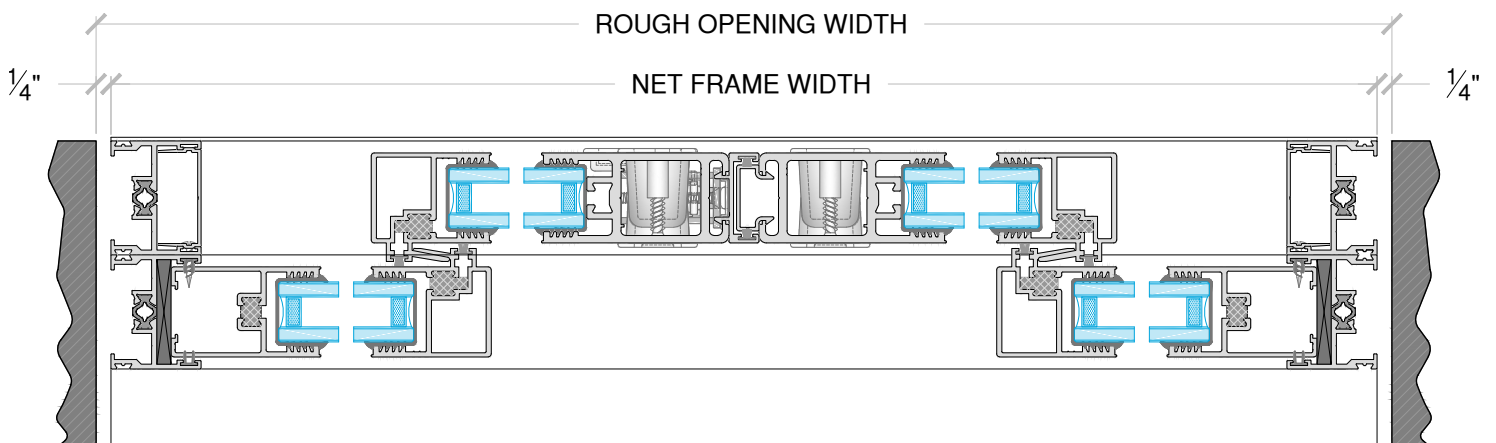
Section
