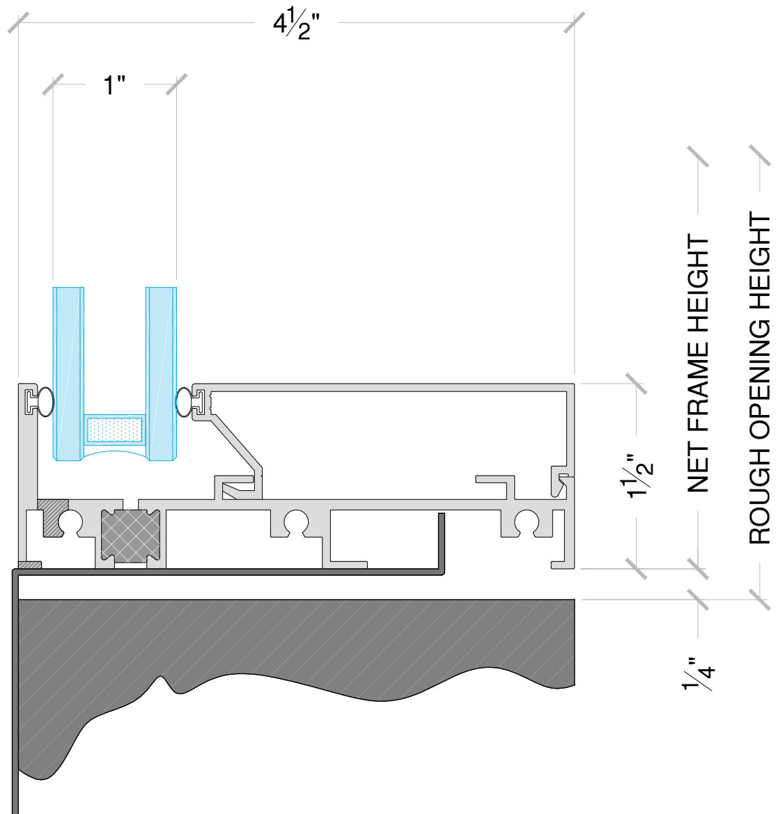
Window Wall Sill - Single Lite
